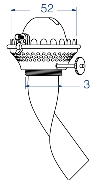
Burner 1''' Type: Flat wick Wick: 25 x 230
