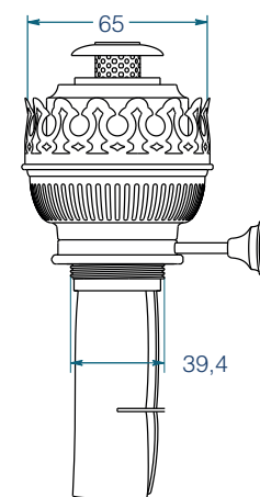
Burner 20''' Type: Ideal burner Wick: 90 x 230
