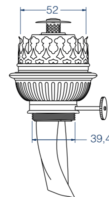
Burner 15''' Type: Round, Odin Wick: 65 x 230
