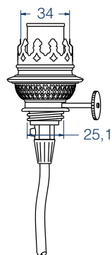
Imitation Burner 6''' Lamp-holder E14
