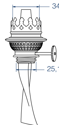
Burner 6''' Type: Round Wick: 35 x 230
