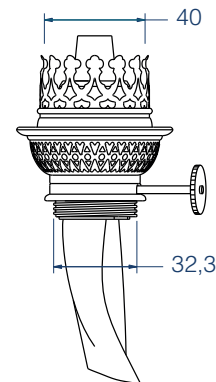
Burner 10''' Type: Round Wick: 48 x 230
