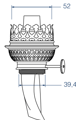
Burner 14''' Type: Round Wick: 65 x 230
